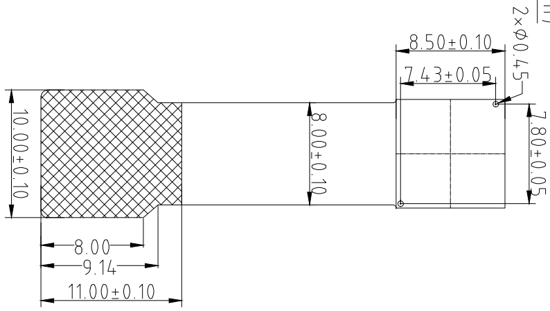
BOTTOM VIEW
